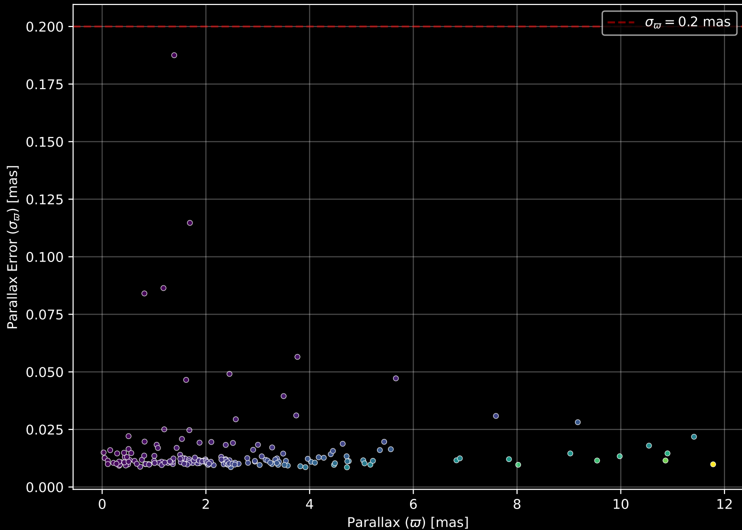
APOGEE DR17 Field: [289-33-O_TESS] Parallax Quality (n= 182)
