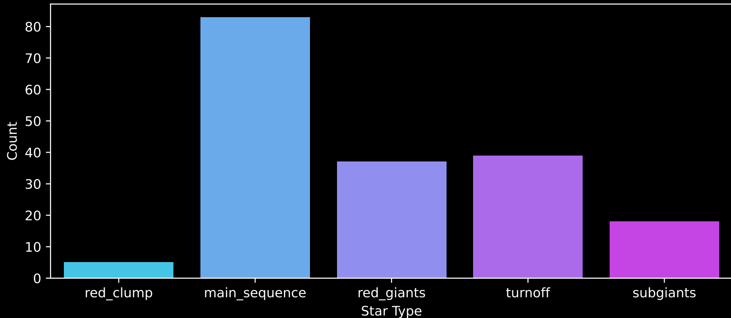
APOGEE DR17 Field: [289-33-O_TESS] Count plot of Star Type
