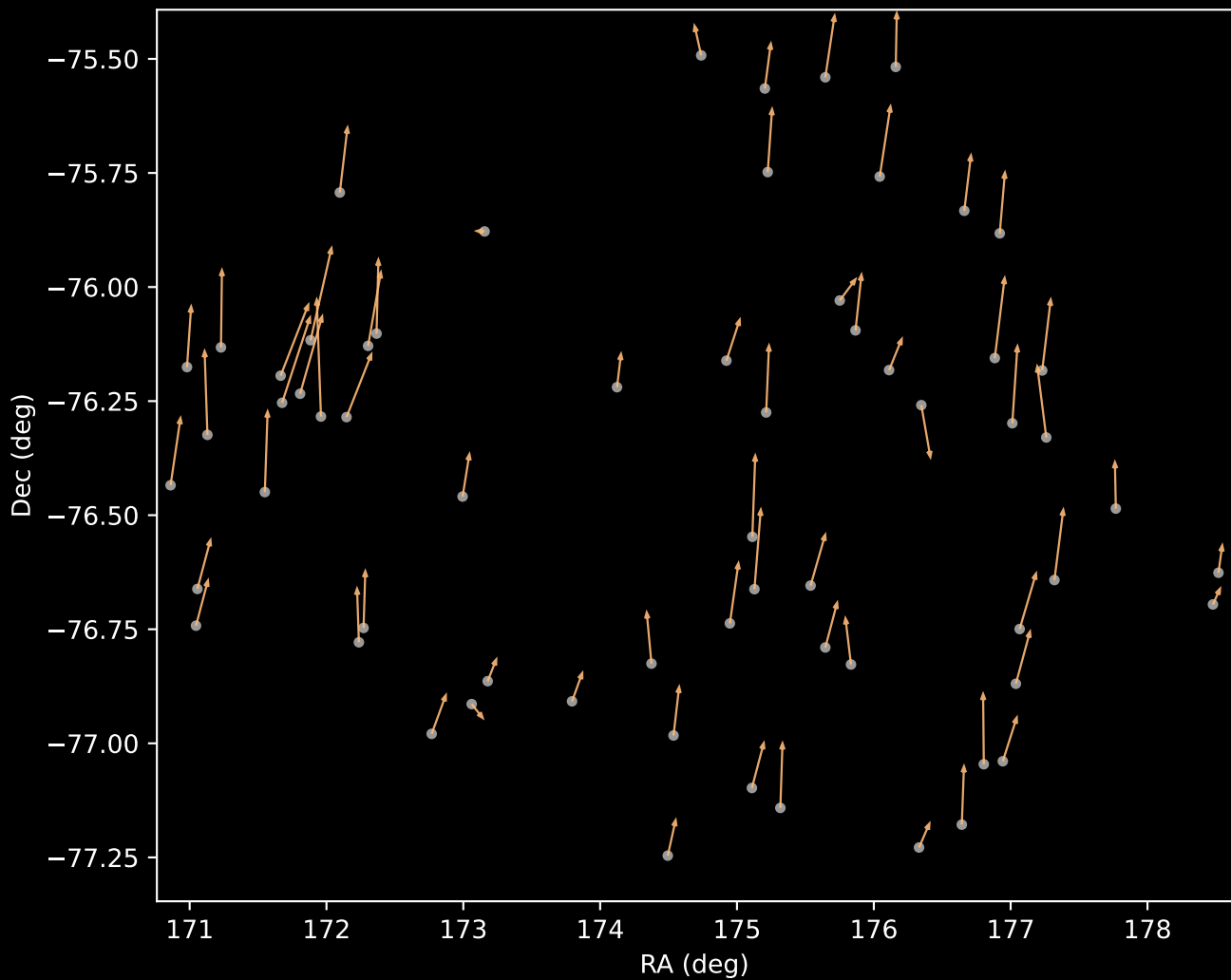
APOGEE DR17 Cluster 3 Proper Motion Vectors (n=64)
