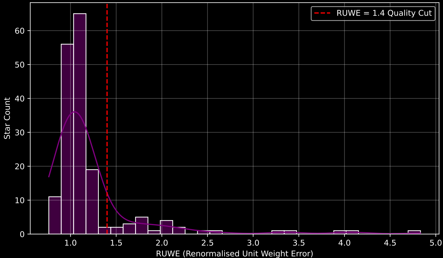
GAPOGEE DR17 Field [289-33-O_TESS] RUWE Distribution (n= 177)
